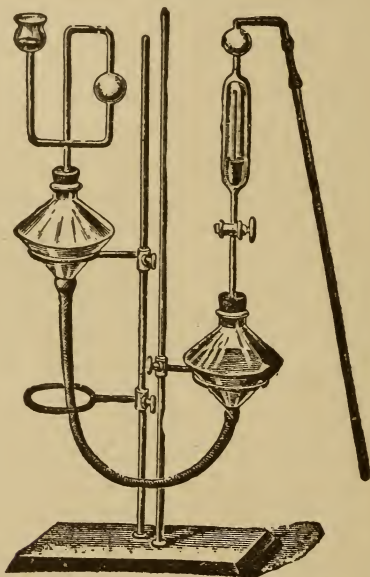
Fig. 104. KAEHLER'S GAS GENERATOR, FOR MAKING CHLORINE.
